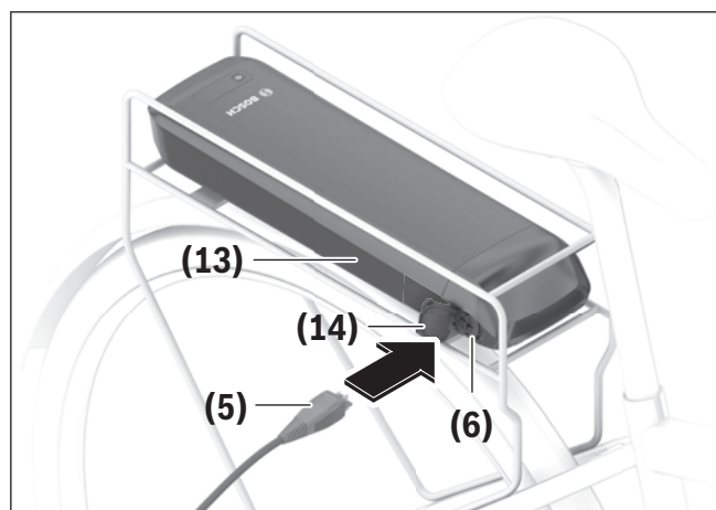
(5) Charging connector
