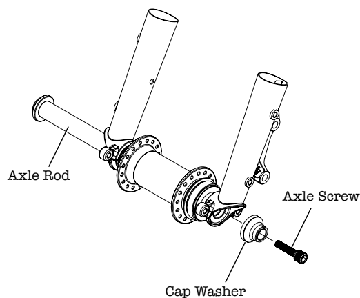
Front Axle Assembly
