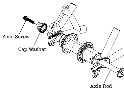
Rear Axle Assembly
